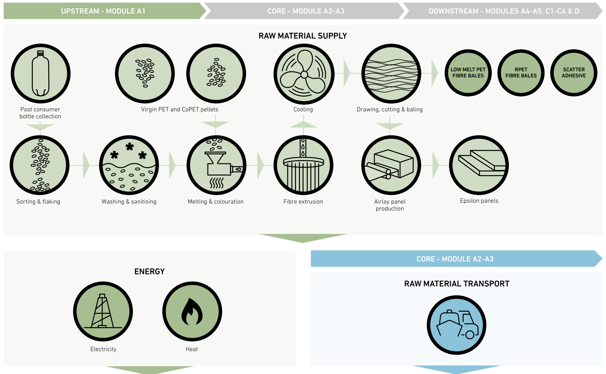
Figure 2: Embossed Panel lifecycle system boundary
