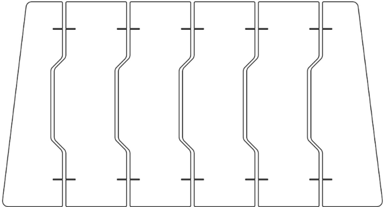
Female End Piece x 1 1750 x 513.5mm
