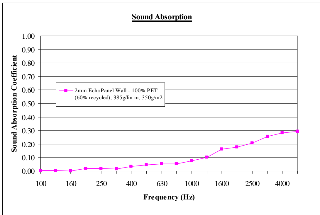
Graph 1: Sound Absorption Coefficients of 2mm EchoPanel Wall (100% PET (60% recycled), 385g/lin m, 350g/m2) tested with no air gap.
