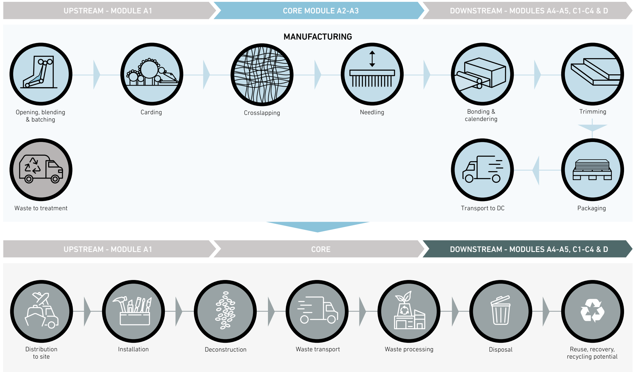
Figure 2 (continued): EchoPanel® 24mm Precision Cut panels lifecycle system boundary
